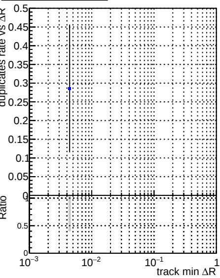
Fake rate vs \Delta R(\text{track, jet}) Duplicates Rate vs \Delta R(\text{track, jet}) Pileup rate vs \Delta R(\text{track, jet}) Legend: DQM_V0001_R000000001 Global CMSSW_ckfnocut3_RECO DQM_V0001_R000000001 Global CMSSW_mknocut3_RECO DQM_V0001_R000000001 Global CMSSW_mknocut3clean3_RECO
