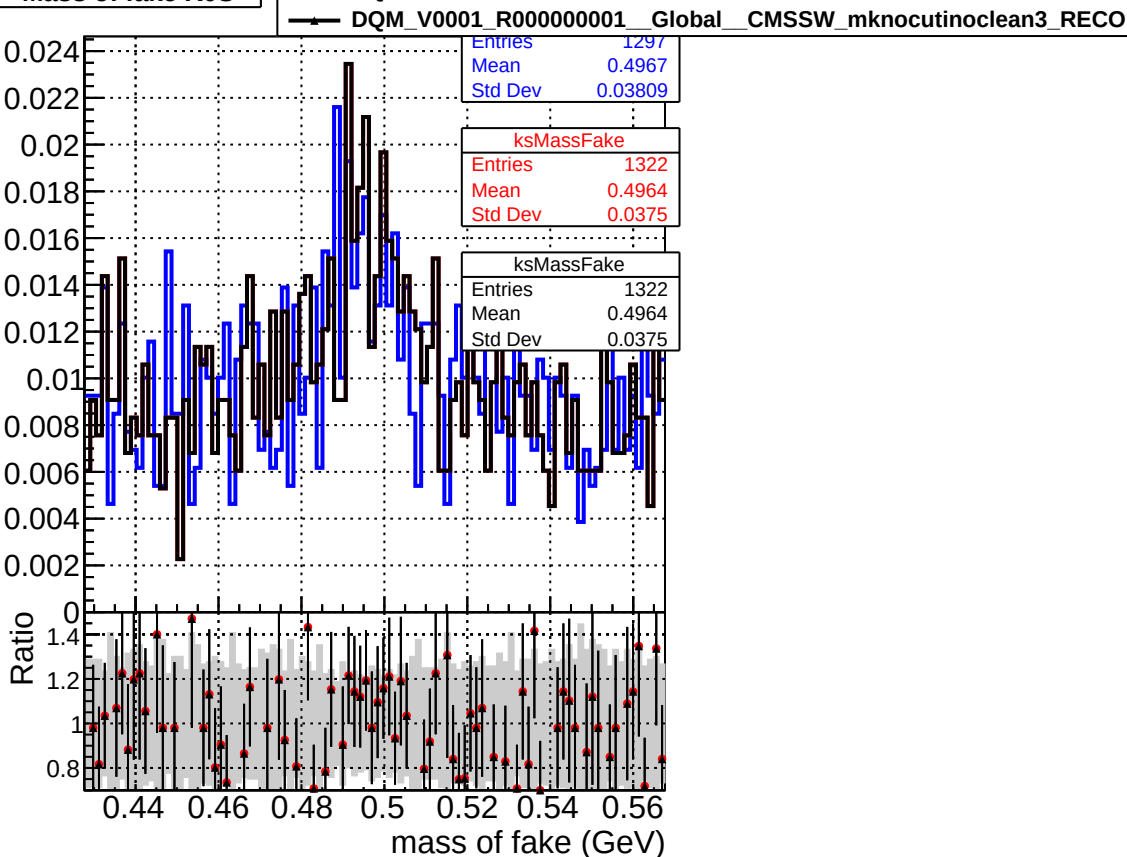
Mass of fake K0S
