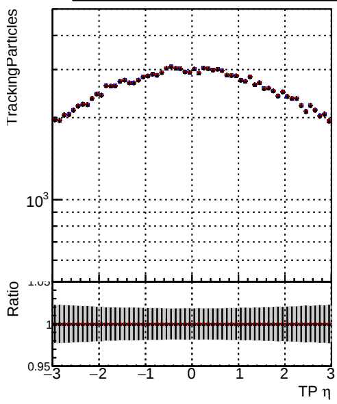
—●— DQM_V0001_R0000000001_Global_CMSSW_ckfnocut3_RECO —●— DQM_V0001_R0000000001_Global_CMSSW_mknocut3_RECO —●— DQM_V0001_R0000000001_Global_CMSSW_mknocut3clean3_RECO
