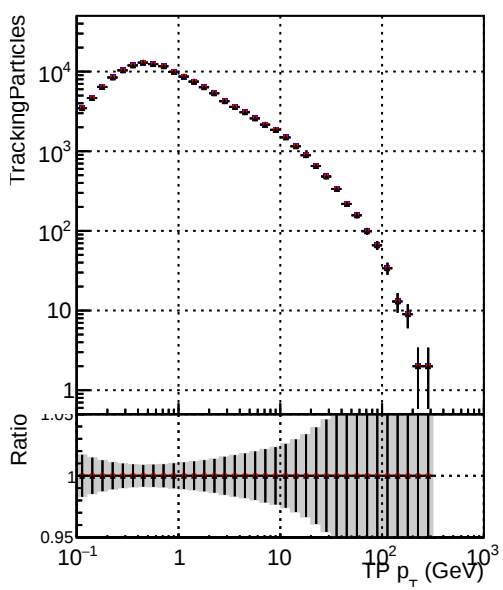
—●— DQM_V0001_R0000000001_Global_CMSSW_ckfnocut3_RECO —●— DQM_V0001_R0000000001_Global_CMSSW_mknocut3_RECO —●— DQM_V0001_R0000000001_Global_CMSSW_mknocut3clean3_RECO
