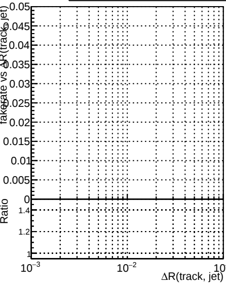
Fake rate vs \Delta R(\text{track}, \text{jet}) Legend: DQM_V0001_R000000001_Global_CMSSW_ckfnocut3_RECO DQM_V0001_R000000001_Global_CMSSW_mknocut3_RECO DQM_V0001_R000000001_Global_CMSSW_mknocutinoclean3_RECO
