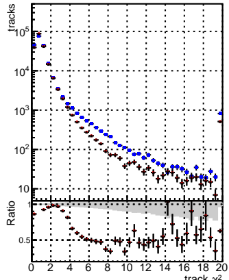
N of reco track vs. \chi^2 Global CMSSW_43mcuc3 RECO Global CMSSW_mknocut3 RECO Global CMSSW_mknocutinoclean3 RECO
