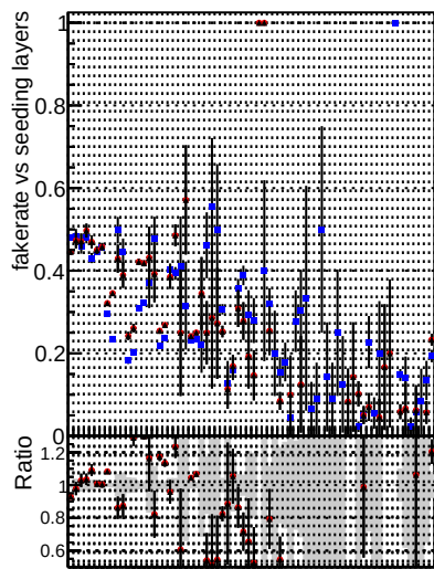
Fake rate vs. DOM V0001 R0000000001 Global CMSSW-ckmcut3-RECO DOM V0001 R0000000001 Global CMSSW-mknocut3-RECO DOM V0001 R0000000001 Global CMSSW-mknocut3clean-RECO
