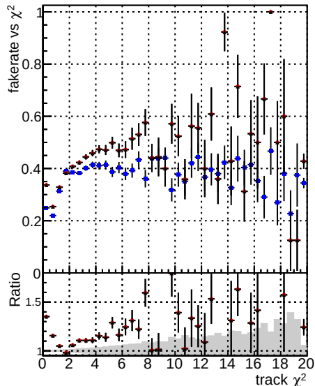
Fake rate vs. DOM V0001 R0000000001 Global CMSSW-ckmcut3-RECO DOM V0001 R0000000001 Global CMSSW-mknocut3-RECO DOM V0001 R0000000001 Global CMSSW-mknocut3clean-RECO
