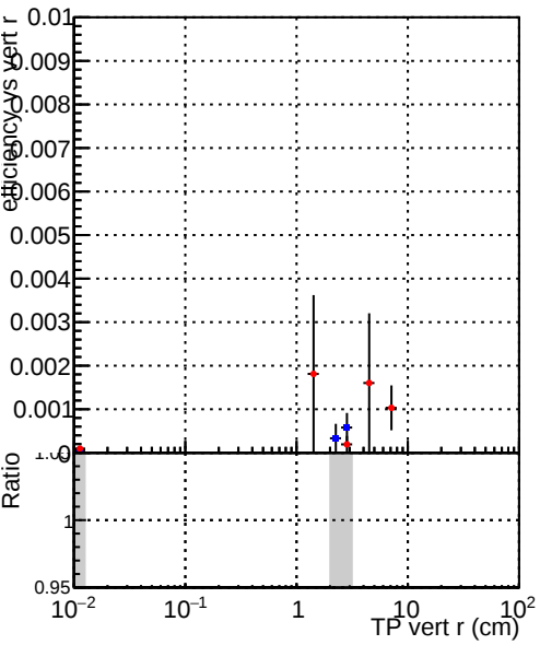
Efficiency vs vertpos Legend: DQM_V0001_R000000001_Global_CMSSW_cknocut3_RECO DQM_V0001_R000000001_Global_CMSSW_mknocut3_RECO
