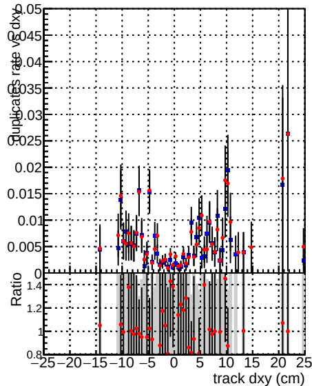
—●— DQM V0001 R0000000001 Global CMSSW_ckptnucut3 RECO —●— DQM V0001 R0000000001 Global CMSSW_mknucut3 RECO
