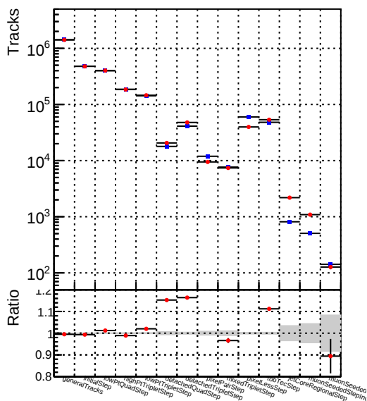
Number of tracks vs collection Legend: Blue dots: DQM_V0001_R000000001_Global_CMSSW_cknocut3_RECO Red dots: DQM_V0001_R000000001_Global_CMSSW_mknocut3_RECO
