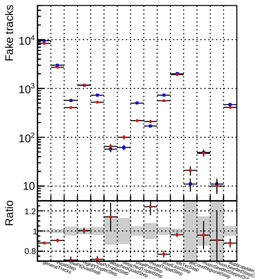
Number —●— DQM_V0001 R000000001 Global CMSSW mknocut3 RECO
