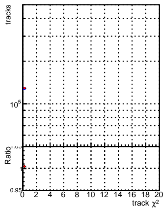
N of reco track vs. \chi^2 for DQM_V0001_R000000001_Global_CMSSW_ckfnocut3_RECO (blue) and DQM_V0001_R000000001_Global_CMSSW_mknocut3_RECO (red).
