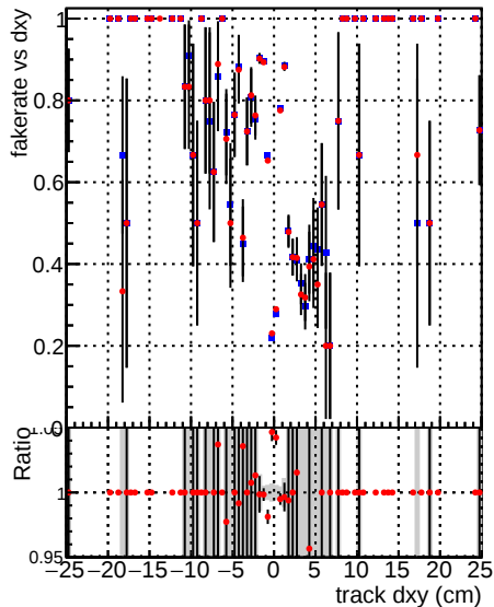
—■— DQM_V0001_R0000000001 Global CMSSW_ckptocut3 RECO —●— DQM_V0001_R0000000001 Global CMSSW_mknocut3 RECO
