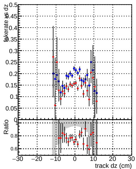
Fake rate vs d —●— DQM V0001_R000000001 Global CMSSW_ckfnocut3 RECO —●— DQM V0001_R000000001 Global CMSSW_mknocut3 RECO
