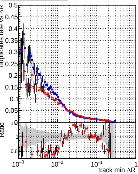
Legend: DQM_V0001_R000000001_Global_CMSSW_ckfnocut3_RECO (blue line with points), DQM_V0001_R000000001_Global_CMSSW_mknocut3_RECO (red line with points)
