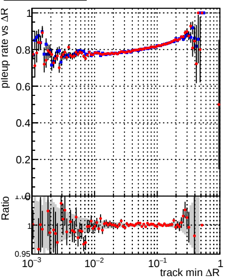
Legend: DQM_V0001_R000000001_Global_CMSSW_ckfnocut3_RECO (blue line with points), DQM_V0001_R000000001_Global_CMSSW_mknocut3_RECO (red line with points)
