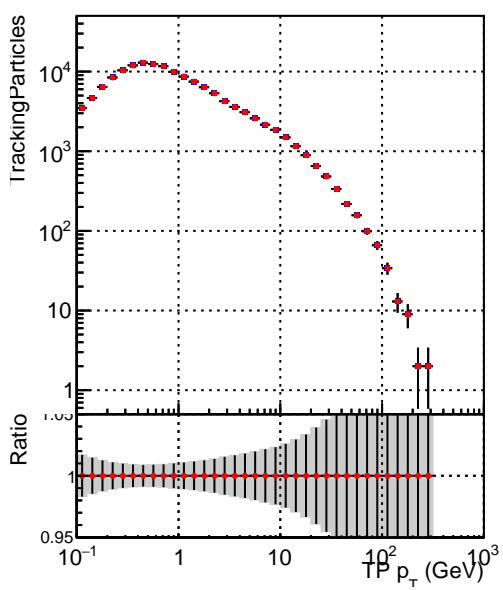
Legend: DQM_V0001_R000000001_Global_CMSSW_ckfnocut3_RECO (blue dots), DQM_V0001_R000000001_Global_CMSSW_mknocut3_RECO (red dots)
