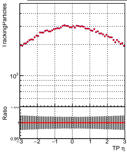
Legend: DQM_V0001_R000000001_Global_CMSSW_ckfnocut3_RECO (blue dots), DQM_V0001_R000000001_Global_CMSSW_mknocut3_RECO (red dots)
