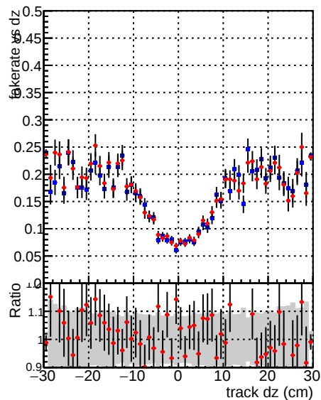
—●— DQM_V0001_R0000000001_Global_CMSSW_ckptocut3_RECO —●— DQM_V0001_R0000000001_Global_CMSSW_mknocut3_RECO
