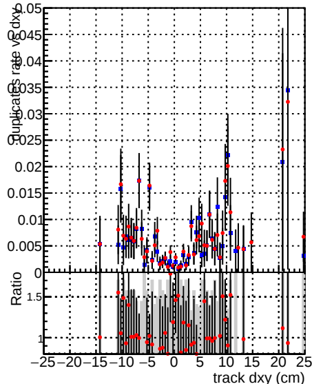
—●— DQM_V0001_R0000000001_Global_CMSSW_ckptocut3_RECO —●— DQM_V0001_R0000000001_Global_CMSSW_mknocut3_RECO
