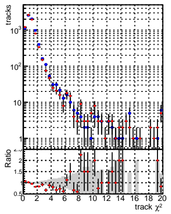
N of reco track vs. \chi^2 Global_CMSSW_ckfnocut3_RECO Global_CMSSW_mknocut3_RECO
