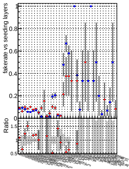
Fake rate vs. —●— DQM V0001_R000000001 Global CMSSW_ckfnocut3 RECO —●— DQM V0001_R000000001 Global CMSSW_mknocut3 RECO
