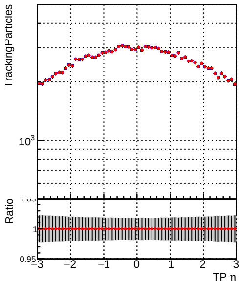
—•— DQM_V0001_R000000001_Global_CMSSW_cknocut3_RECO —•— DQM_V0001_R000000001_Global_CMSSW_mknocut3_RECO
