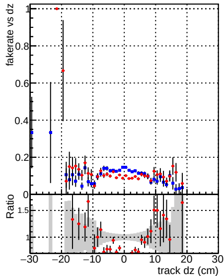
Fake rate vs dz Global CMSSW_ckptocut3 RECO Global CMSSW_mknocut3 RECO
