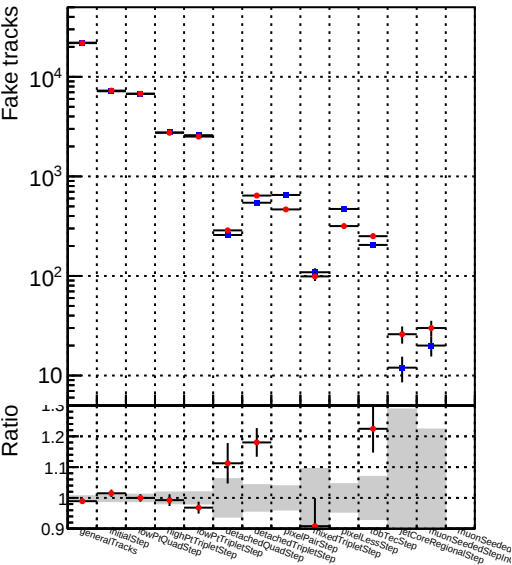
Number ● DQM_V0001_R000000001_Global_CMSSW_mknocut3_RECO
