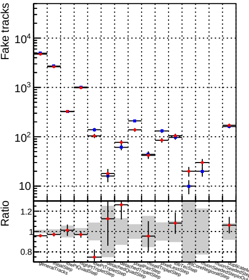
Number ● DQM_V0001_R000000001_Global_CMSSW_mknocut3_RECO
