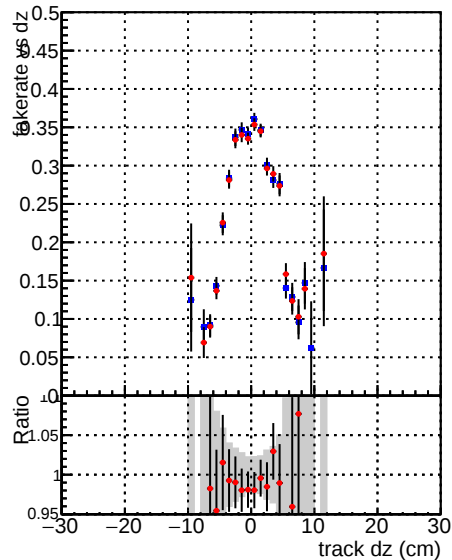
—●— DQM_V0001_R0000000001_Global_CMSSW_ckfnocut3_RECO —●— DQM_V0001_R0000000001_Global_CMSSW_mknocut3_RECO
