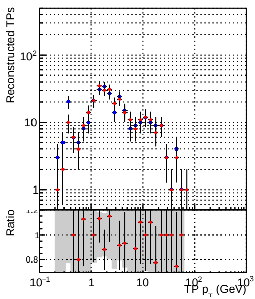
—•— DQM_V0001_R0000000001_Global_CMSSW_cknocut3_RECO —•— DQM_V0001_R0000000001_Global_CMSSW_mknocut3_RECO
