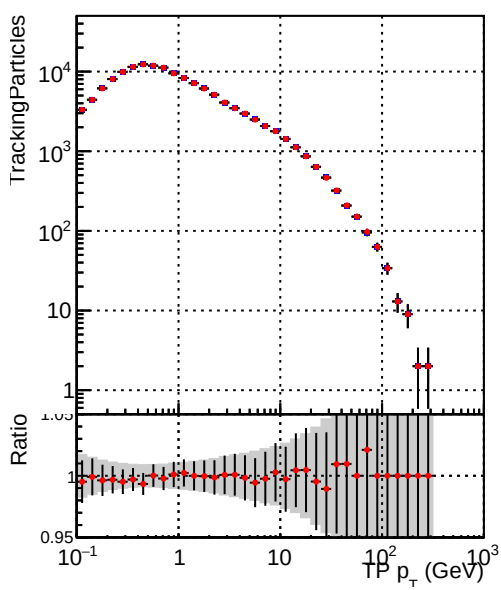
—•— DQM_V0001_R0000000001_Global_CMSSW_cknocut3_RECO —•— DQM_V0001_R0000000001_Global_CMSSW_mknocut3_RECO
