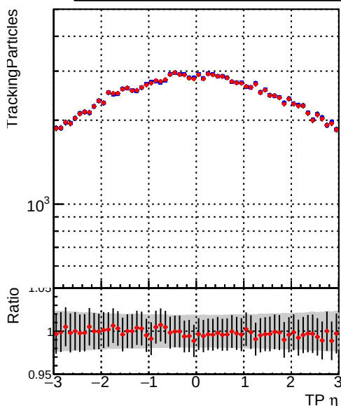
—•— DQM_V0001_R0000000001_Global_CMSSW_cknocut3_RECO —•— DQM_V0001_R0000000001_Global_CMSSW_mknocut3_RECO
