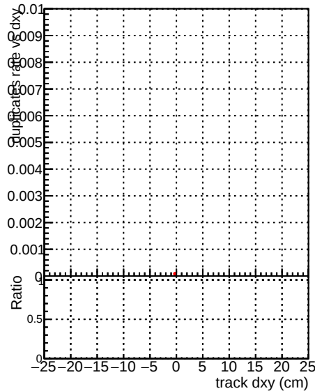
—●— DQM_V0001_R0000000001 —●— DQM_V0001_R0000000001 —●— Global —●— Global —●— CMSSW_ckfnocut3_RECO —●— CMSSW_mknocut3_RECO
