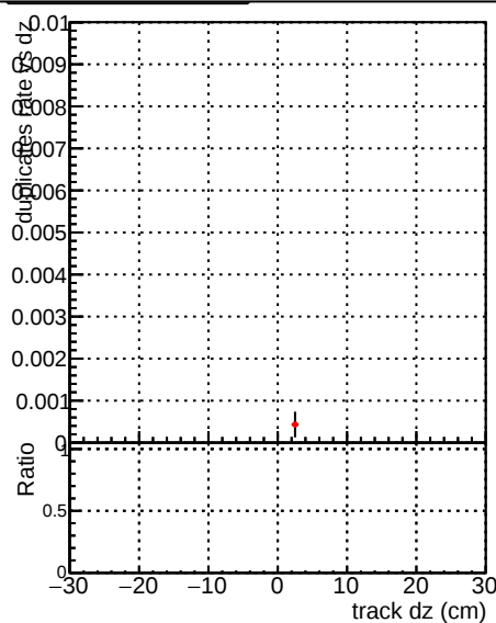
—●— DQM_V0001_R0000000001 —●— DQM_V0001_R0000000001 —●— Global —●— Global —●— CMSSW_ckfnocut3_RECO —●— CMSSW_mknocut3_RECO
