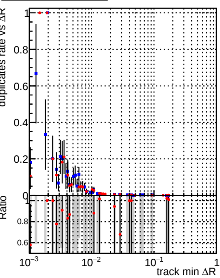
Legend: DQM_V0001_R000000001_Global_CMSSW_ckfnocut3_RECO (blue squares), DQM_V0001_R000000001_Global_CMSSW_mknocut3_RECO (red circles)
