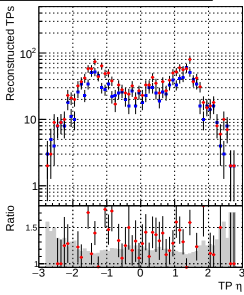
Legend: ■ DQM_V0001_R0000000001_Global_CMSSW_cknocut3_RECO ■ DQM_V0001_R0000000001_Global_CMSSW_mknocut3_RECO
