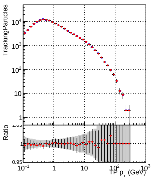
Legend: ■ DQM_V0001_R0000000001_Global_CMSSW_cknocut3_RECO ■ DQM_V0001_R0000000001_Global_CMSSW_mknocut3_RECO
