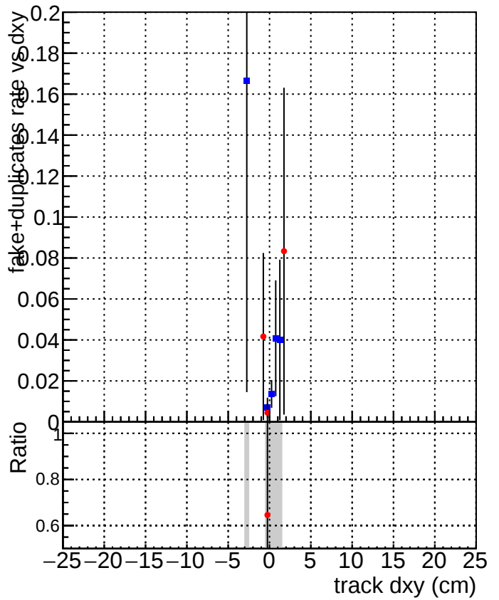
DQM_V0001_R000000001_Global_CMSSW_ckfnocut3_RECO DQM_V0001_R000000001_Global_CMSSW_mknocut3_RECO
