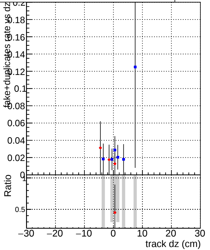
DQM_V0001_R000000001_Global_CMSSW_ckfnocut3_RECO DQM_V0001_R000000001_Global_CMSSW_mknocut3_RECO
