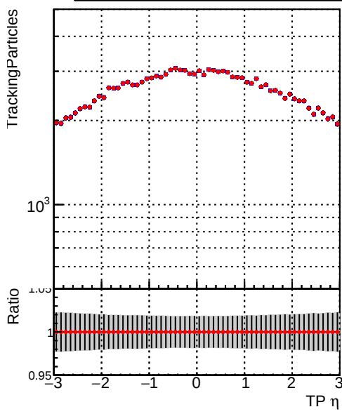
—•— DQM_V0001_R0000000001_Global_CMSSW_cknocut3_RECO —•— DQM_V0001_R0000000001_Global_CMSSW_mknocut3_RECO
