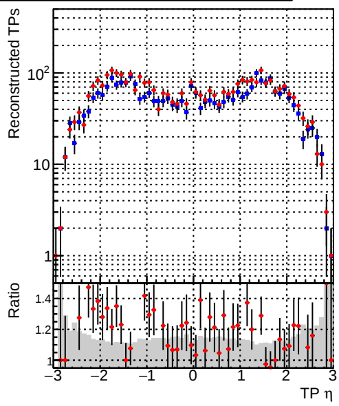
—•— DQM_V0001_R0000000001_Global_CMSSW_cknocut3_RECO —•— DQM_V0001_R0000000001_Global_CMSSW_mknocut3_RECO
