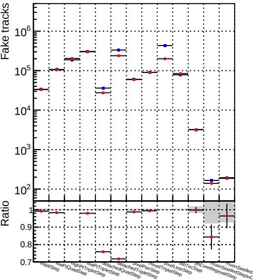
Numbe —●— DQM_V0001_R000000001_Global_CMSSW_mknocut3_RECO
