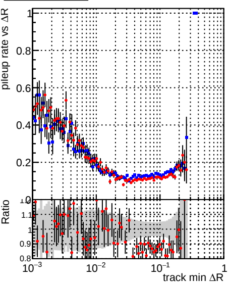
Legend: \Delta R (blue) DQM_V0001_R000000001_Global_CMSSW_ckfnocut3_RECO \Delta R (red) DQM_V0001_R000000001_Global_CMSSW_mknocut3_RECO
