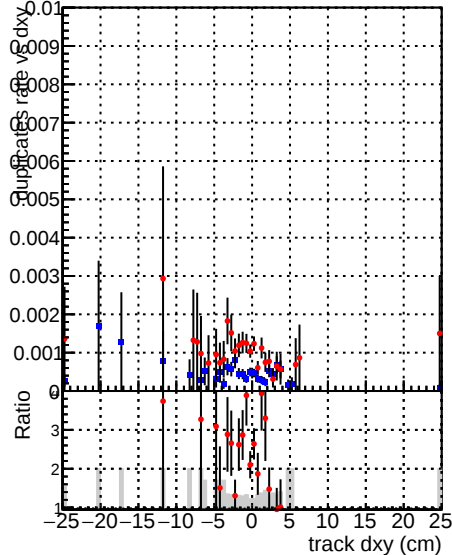
—●— DQM_V0001_R0000000001_Global CMSSW_ckptcut3_RECO —●— DQM_V0001_R0000000001_Global CMSSW_mknocut3_RECO
