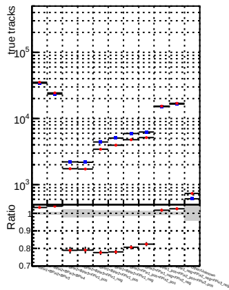
1__Global__CMSSW_mknocut3_RECO
