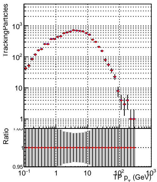
— DQM_V0001_R0000000001_Global_CMSSW_ckfnocut3_RECO — DQM_V0001_R0000000001_Global_CMSSW_mknocut3_RECO
