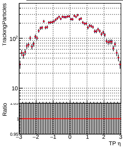
Legend: DQM_V0001_R000000001_Global_CMSSW_cknucut3_RECO (blue line), DQM_V0001_R000000001_Global_CMSSW_mknucut3_RECO (red line)
