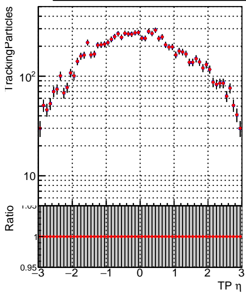
N of simulated tracks vs \eta Legend: — DQM_V0001_R000000001_Global_CMSSW_cknocut3_RECO — DQM_V0001_R000000001_Global_CMSSW_mknocut3_RECO
