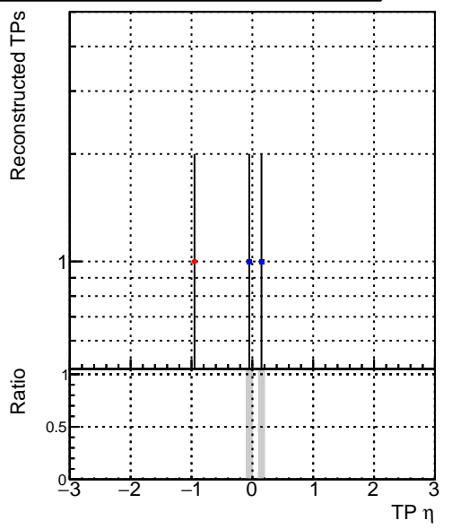
N of simulated tracks vs \eta Legend: — DQM_V0001_R000000001_Global_CMSSW_cknocut3_RECO — DQM_V0001_R000000001_Global_CMSSW_mknocut3_RECO
