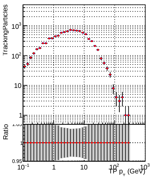
Legend: DQM_V0001_R000000001_Global_CMSSW_cknucut3_RECO (blue diamond), DQM_V0001_R000000001_Global_CMSSW_mknucut3_RECO (red diamond)
