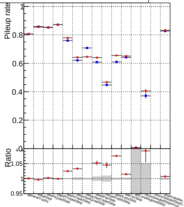
DQM_V0001_R000000001_Global_CMSSW_ckfnocut3_RECO
