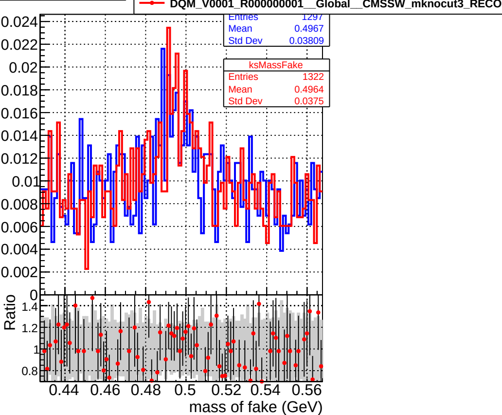
Mass of fake K0S
