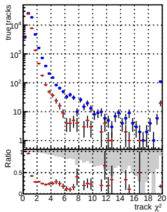
N of reco track vs. —●— DQM_V0001_R0000000001_Global_CMSSW_ckptcut3_RECO —●— DQM_V0001_R0000000001_Global_CMSSW_mknocut3_RECO
