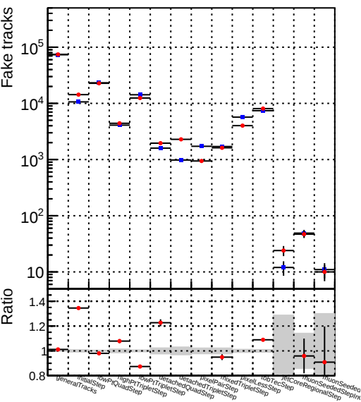
Number ● DQM_V0001_R000000001_Global_CMSSW_mknocut2_RECO
