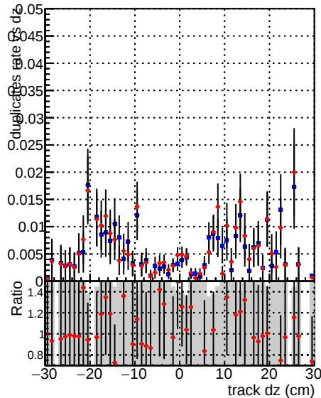
al CMSSW_ ckfnocut2 RECO al CMSSW_ mknocut2 RECO
