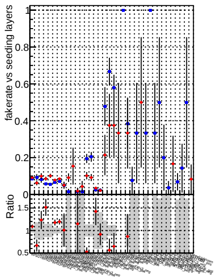
Fake rate vs. Legend Global CMSSW_ckptcut2_RECO Blue diamonds DQM_V0001_R0000000001 CMSSW_ckptcut2_RECO Red diamonds DQM_V0001_R0000000001 CMSSW_mknocut2_RECO
