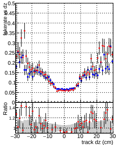
—●— DQM_V0001_R000000001_Global_CMSSW_ckfnocut2_RECO —●— DQM_V0001_R000000001_Global_CMSSW_mknocut2_RECO
