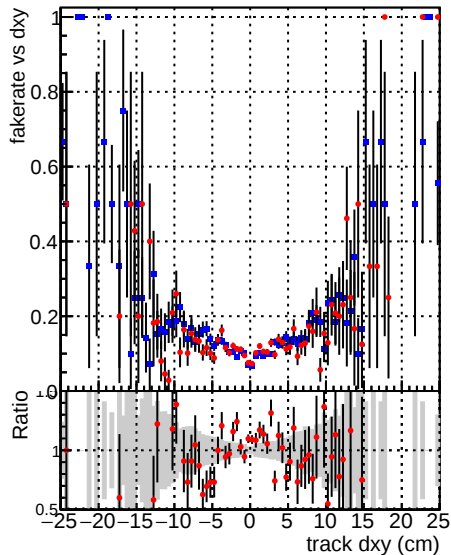
—●— DQM_V0001_R000000001_Global_CMSSW_ckfnocut2_RECO —●— DQM_V0001_R000000001_Global_CMSSW_mknocut2_RECO
