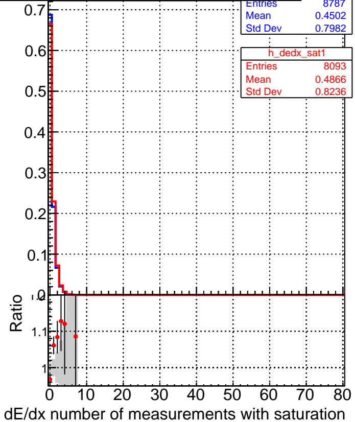
■ DQM_V0001_R000000001_Global_CMSSW_ckfnocut2_RECO ● DQM_V0001_R000000001_Global_CMSSW_mknocut2_RECO
