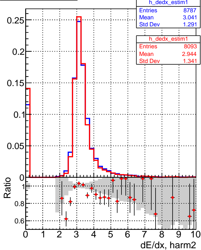
■ DQM_V0001_R000000001_Global_CMSSW_ckfnocut2_RECO ● DQM_V0001_R000000001_Global_CMSSW_mknocut2_RECO
