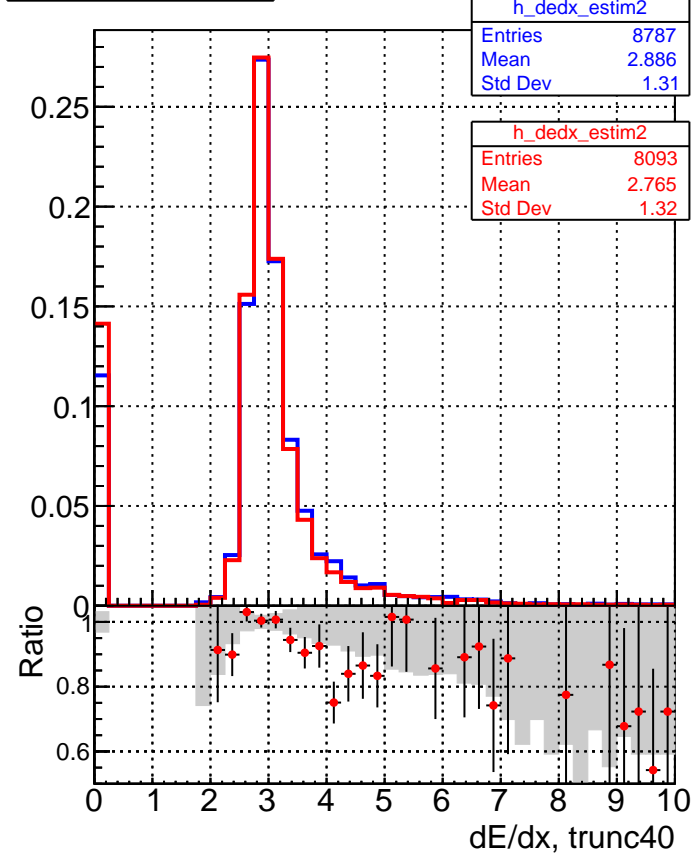
■ DQM_V0001_R000000001_Global_CMSSW_ckfnocut2_RECO ● DQM_V0001_R000000001_Global_CMSSW_mknocut2_RECO
