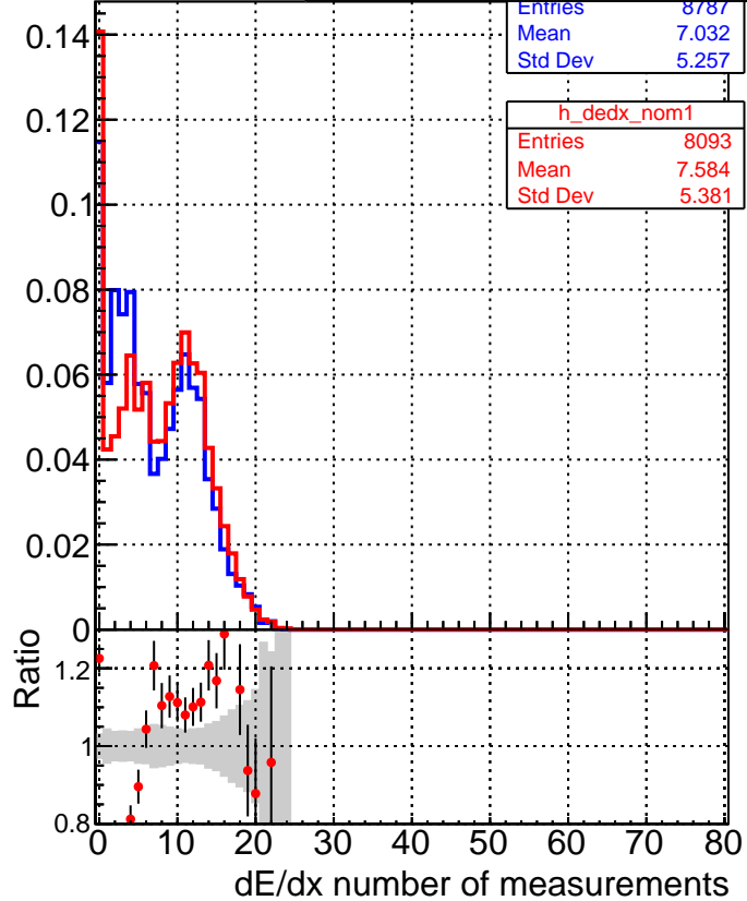
■ DQM_V0001_R000000001_Global_CMSSW_ckfnocut2_RECO ● DQM_V0001_R000000001_Global_CMSSW_mknocut2_RECO
