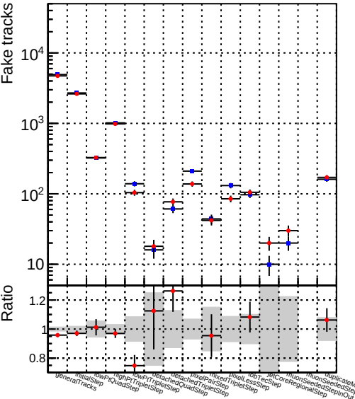
Number ● DQM_V0001_R000000001_Global_CMSSW_mknocut2_RECO
