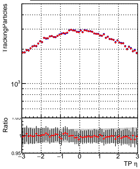
N of simulated tracks vs \eta Legend: — DQM_V0001_R000000001_Global_CMSSW_cknocut2_RECO (blue crosses) — DQM_V0001_R000000001_Global_CMSSW_mknocut2_RECO (red crosses)
