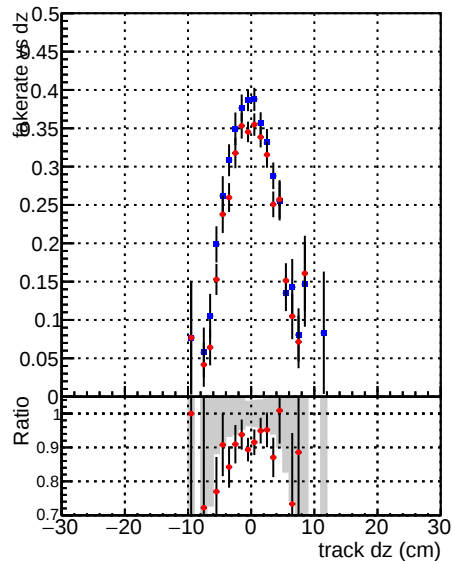
Fake rate vs d DQM_V0001_R0000000001 Global DQM_V0001_R0000000001 Global CMSSW_ckfnocut2 RECO CMSSW_mknocut2 RECO
