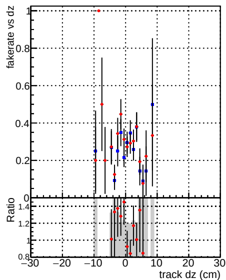
Global CMSSW_ckfnocut2 RECO Global CMSSW_mknocut2 RECO Fake rate vs dz
