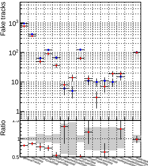
Number ● DQM_V0001_R000000001_Global_CMSSW_mknocut2_RECO
